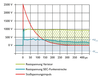
Time curve for a voltage surge pulse
