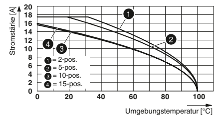
Derating curve
