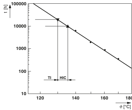
Diagram for extrapolating the TI and HIC value
