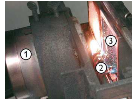
1 Radiant heater 2 Flame 3 Plastic sample
