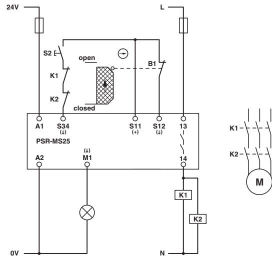
Figure 5 Safety door monitoring/manual, monitored start
