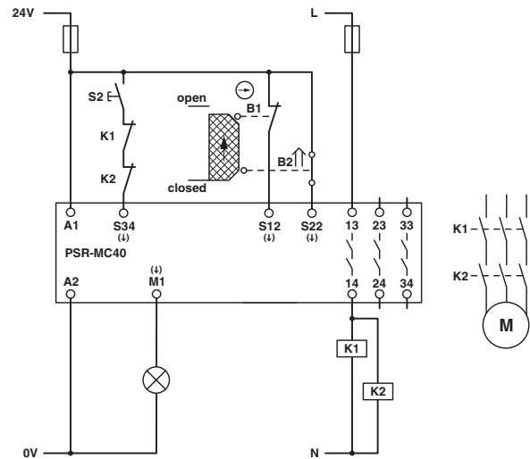
Figure 52 Safety door monitoring/manual, monitored start
