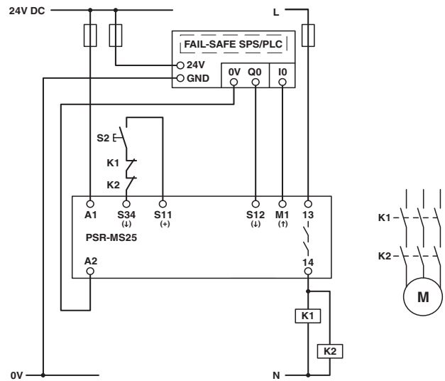
Figure 6 Connection to failsafe PLC/manual, monitored start
