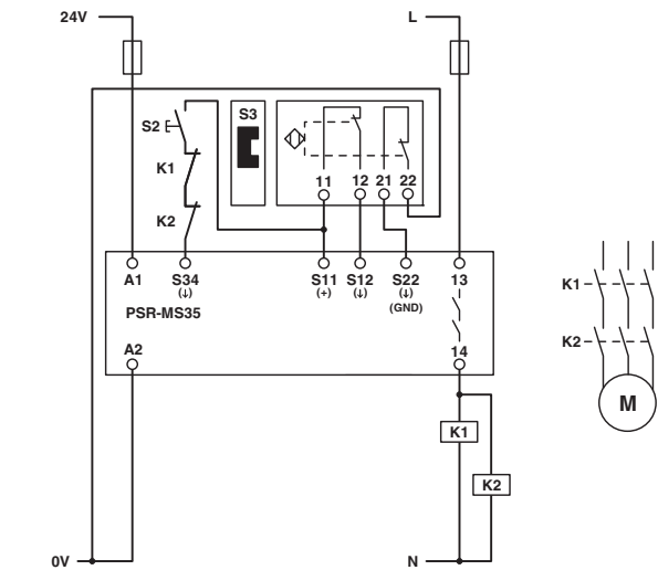
Figure 12 Magnetic switch monitoring/manual, monitored start
