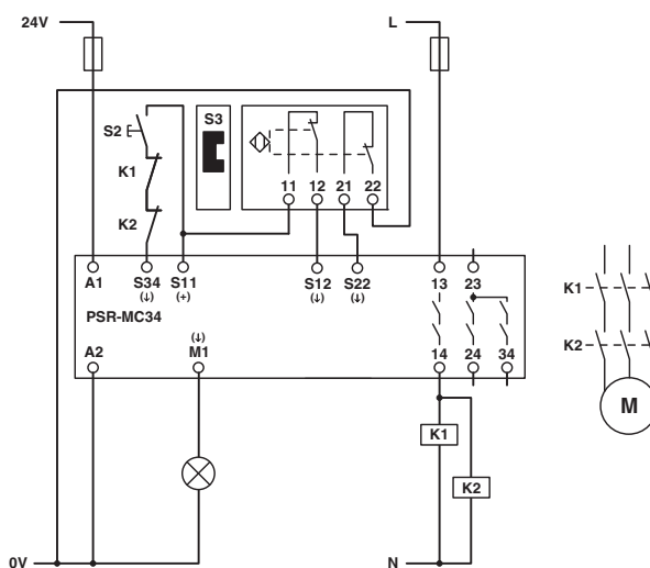
Figure 48 Magnetic switch monitoring/manual, monitored start
